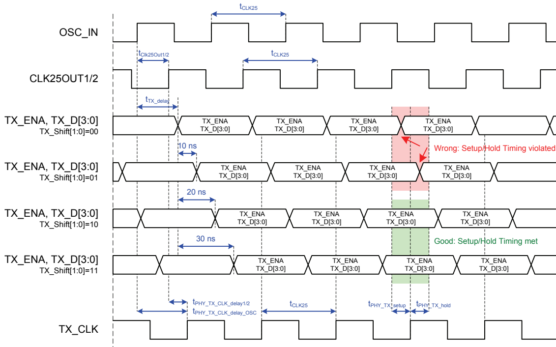
Figure 5: TX Shift Timing Diagram
