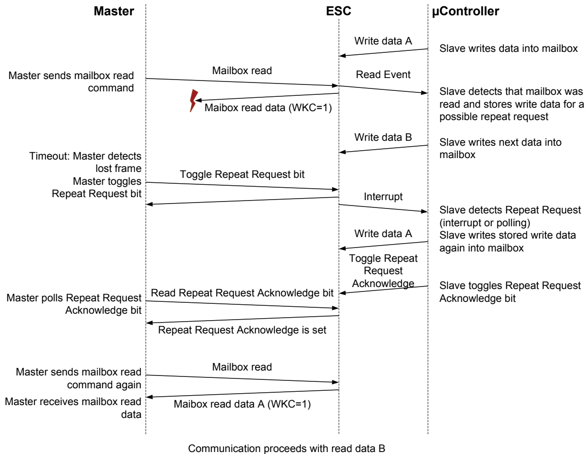
Figure 26: Handling of Write/Read Toggle with Read Mailbox
