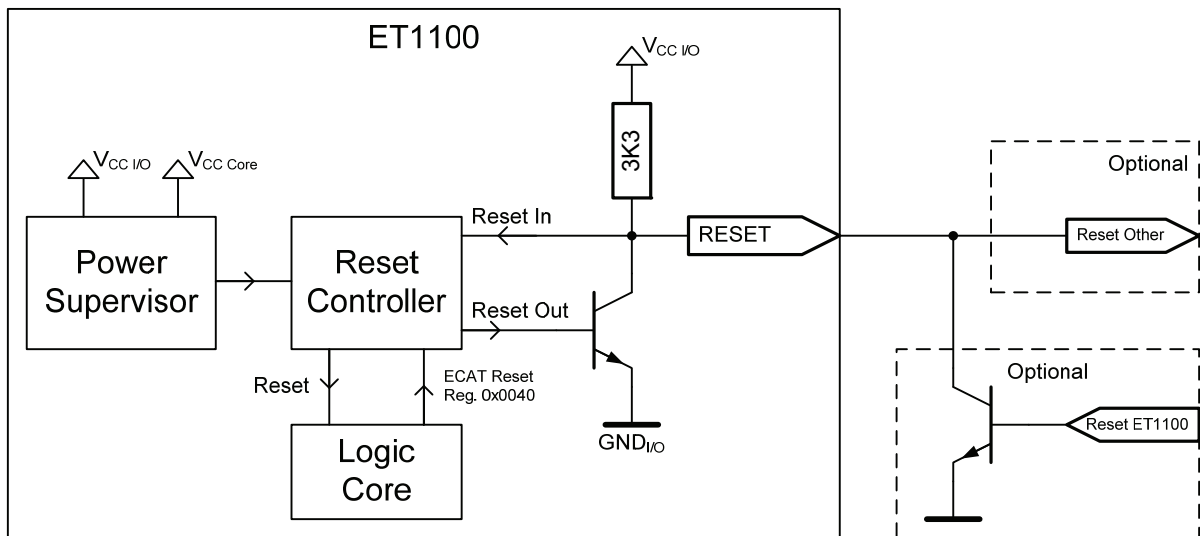
Figure 50: Reset Logic
