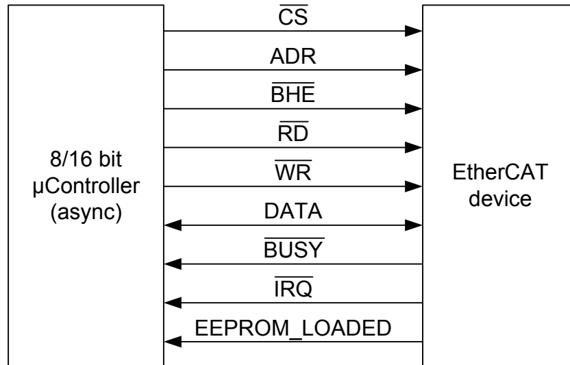
Figure 21: \mu Controller interconnection 3
