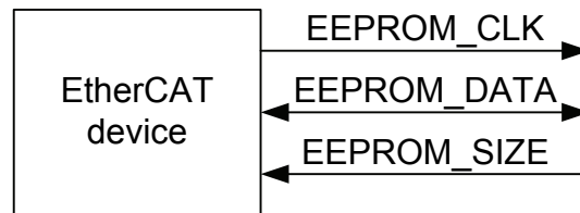
Figure 37: I 2 C EEPROM signals
