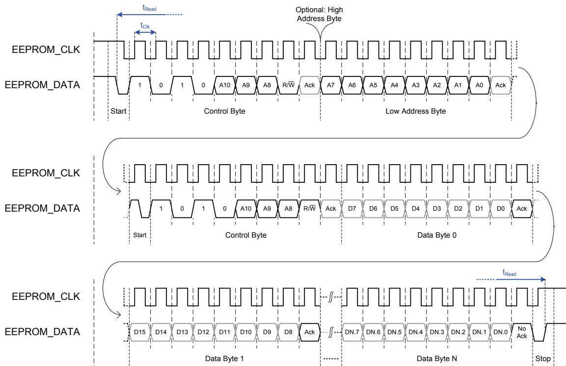
Figure 40: Read access (1 address byte, up to 16 kBit EEPROMs)
