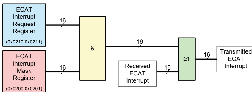
Figure 42: ECAT Interrupt Masking
