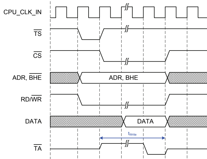
Figure 34: Write access (CS after TS, Write DATA after CS, CS and TA on rising edge)
