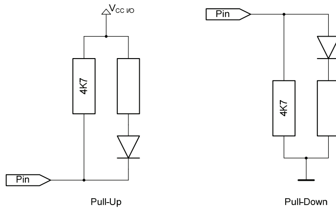
Figure 46: Dual purpose configuration input/LED output pins
