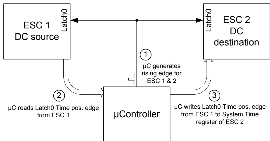
Figure 32: System Time PDI Controlled with three steps
