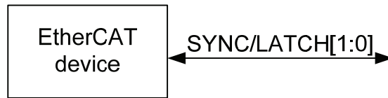
Figure 38: Distributed Clocks signals
