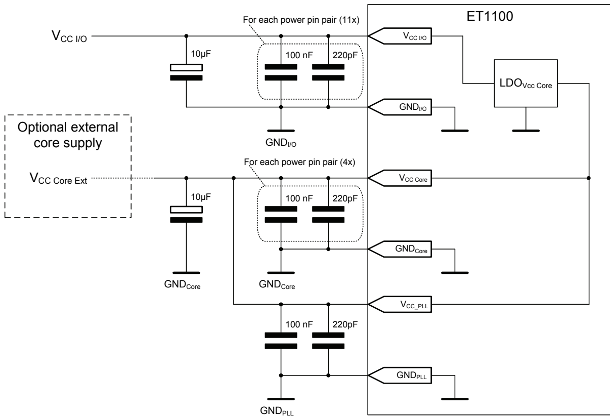
Figure 45: ET1100 power supply
