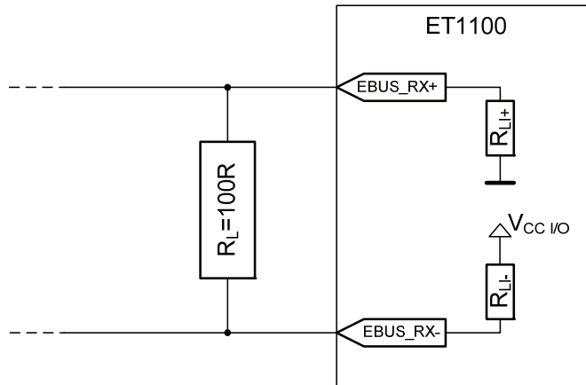
Figure 48: LVDS termination
