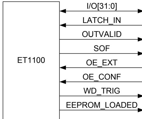
Figure 8: ET1100 Digital I/O signals
