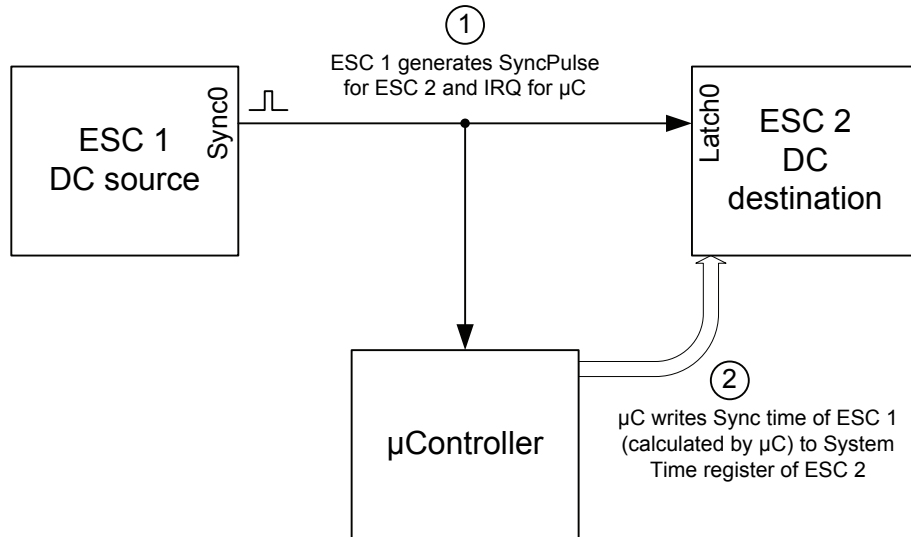
Figure 33: System Time PDI Controlled with two steps
