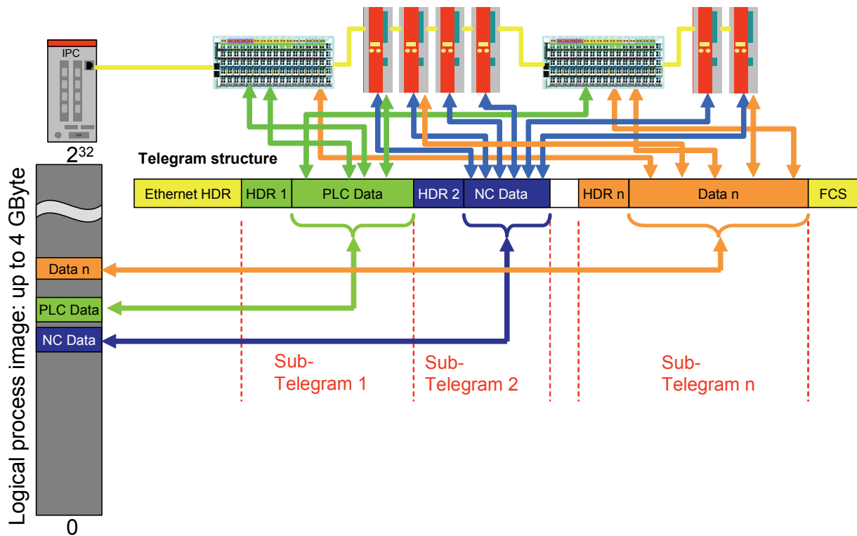
Figure 20: FMMU Mapping Principle
