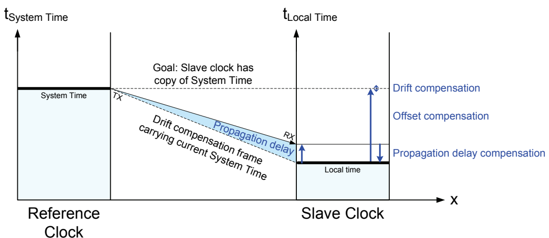
Figure 27: Propagation Delay, Offset, and Drift Compensation
