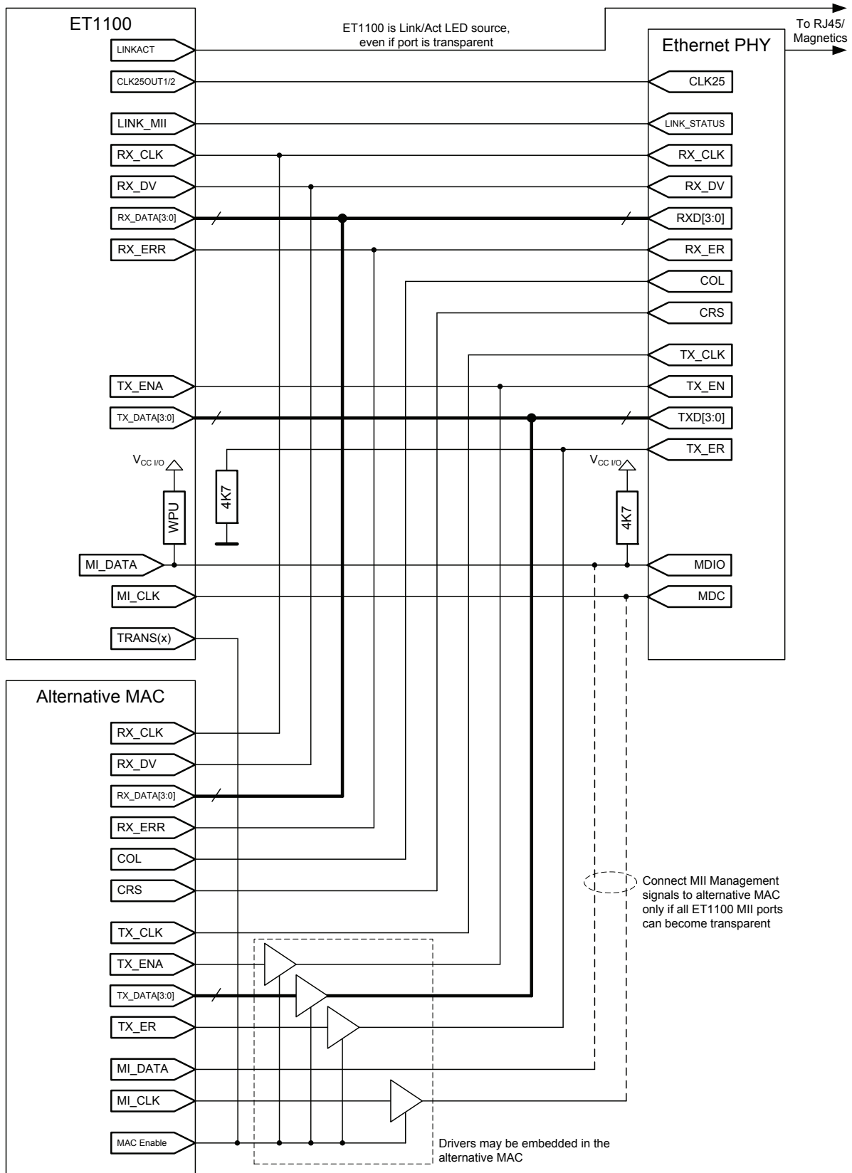
Figure 51: Transparent Mode
