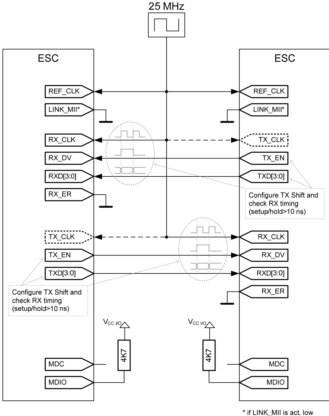
Figure 14: Back-to-Back MII Connection (two ESCs)
