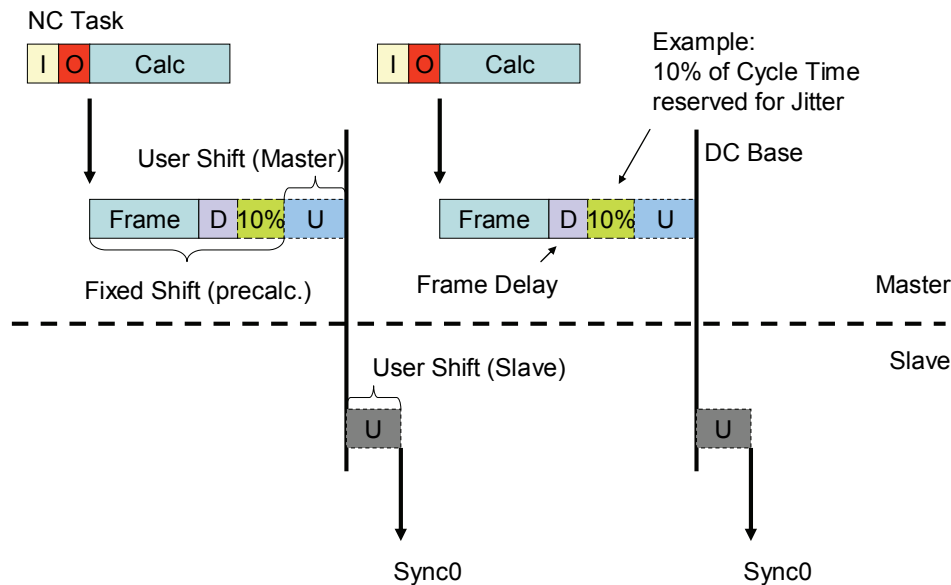
Figure 34: DC Timing Signals in relation to Communication
