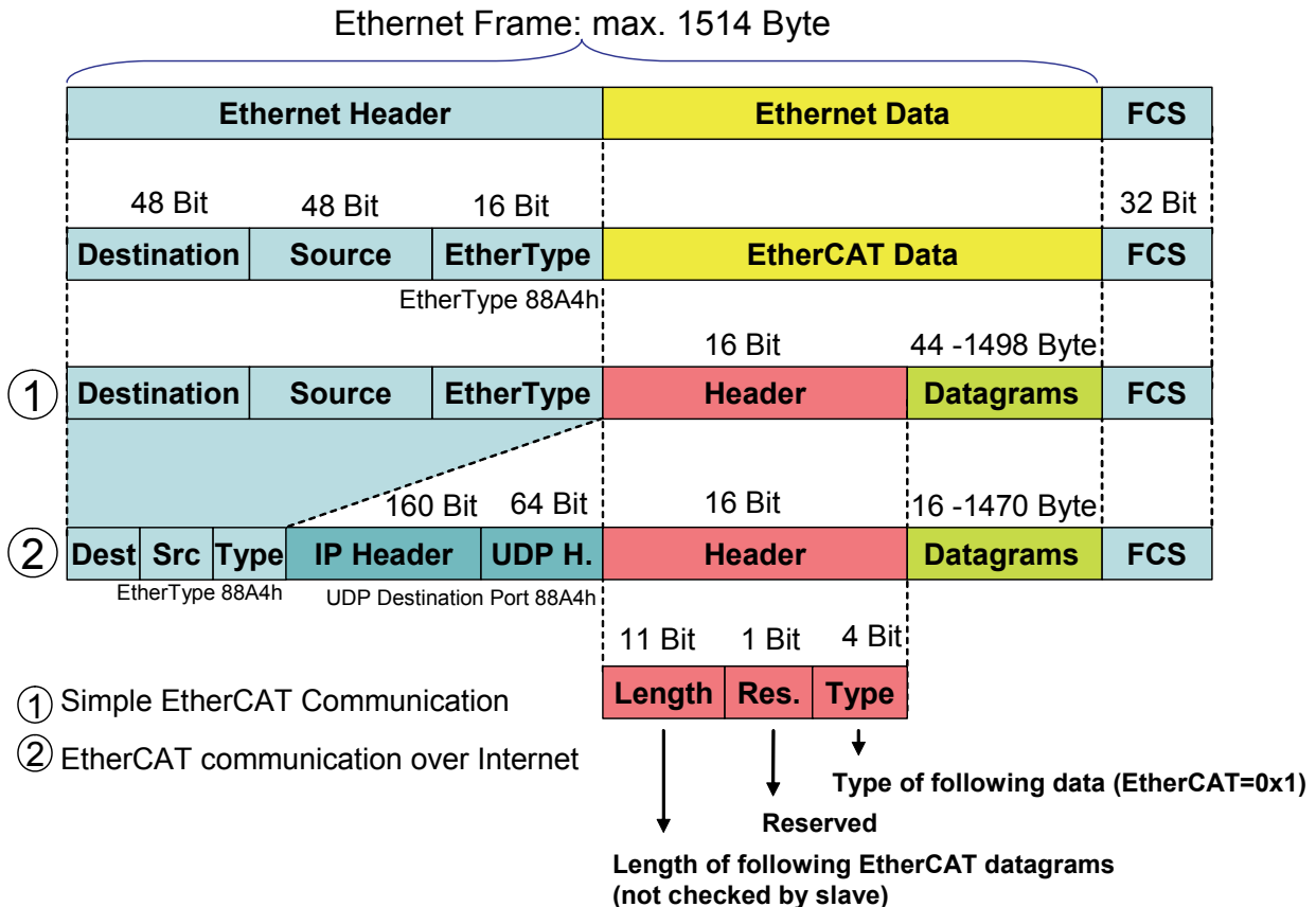
Figure 2: Ethernet Frame with EtherCAT Data
