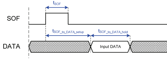
Figure 11: Digital Input: Input data sampled at SOF, I/O can be read in the same frame
