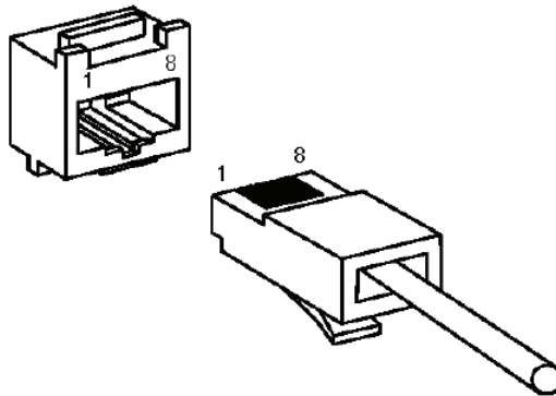
Figure 12: RJ45 Connector
