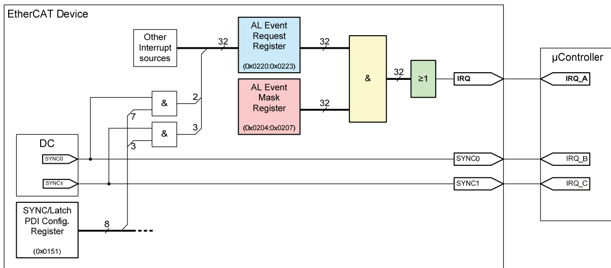
Figure 41: PDI Interrupt Masking and interrupt signals
