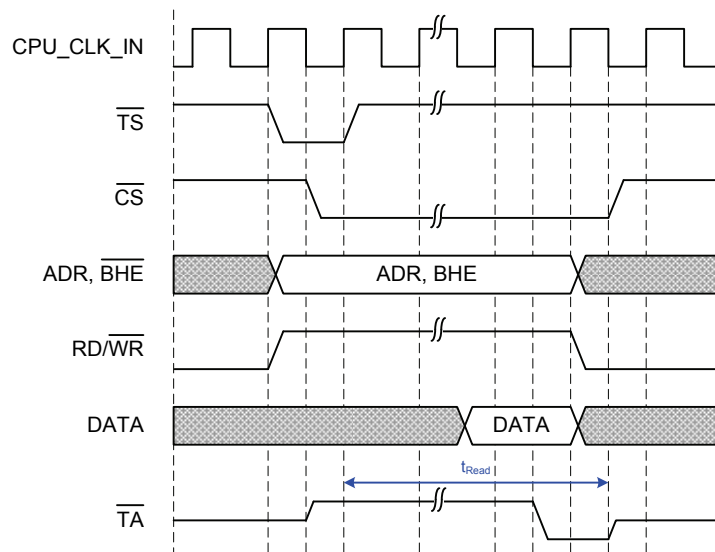
Figure 36: Read access (CS half a clock period after TS, CS and TA on falling edge)
