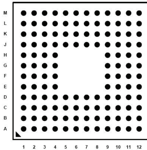
Figure 54: TFBGA 128 Pin Layout
