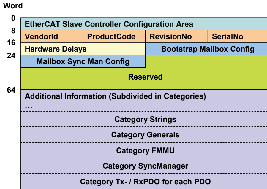
Figure 36: ESI EEPROM Layout
