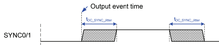
Figure 40: SyncSignal timing
