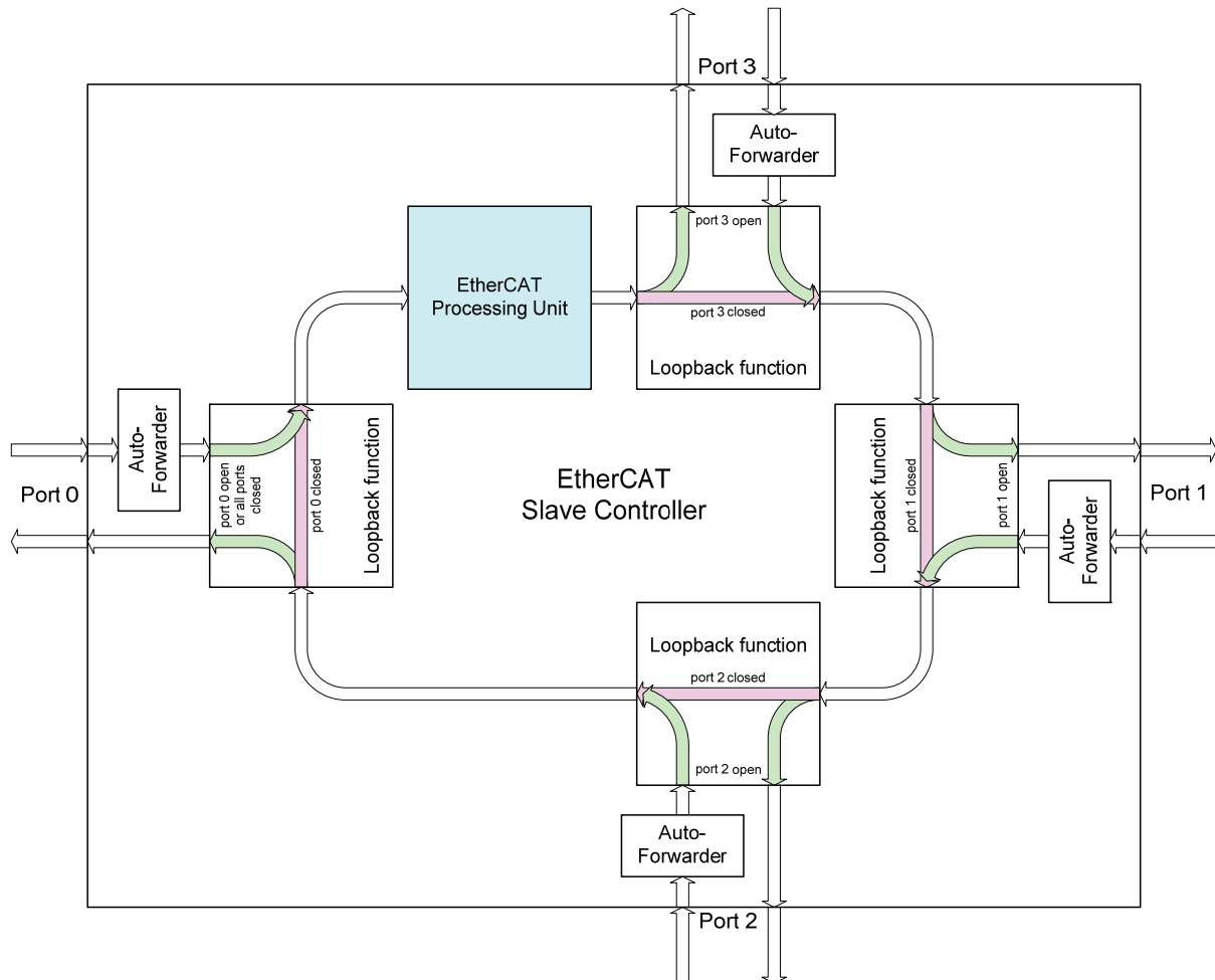
Figure 4: Frame Processing
