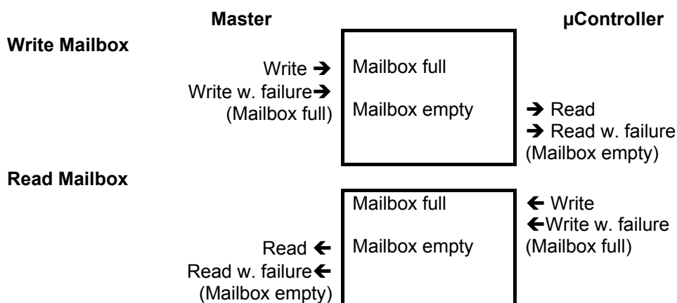
Figure 24: SyncManager Mailbox Interaction
