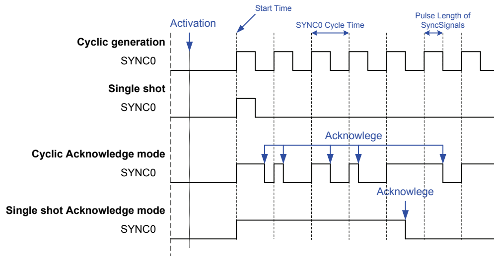
Figure 30: SyncSignal Generation Modes
