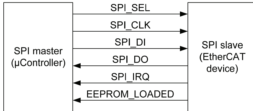
Figure 15: SPI master and slave interconnection
