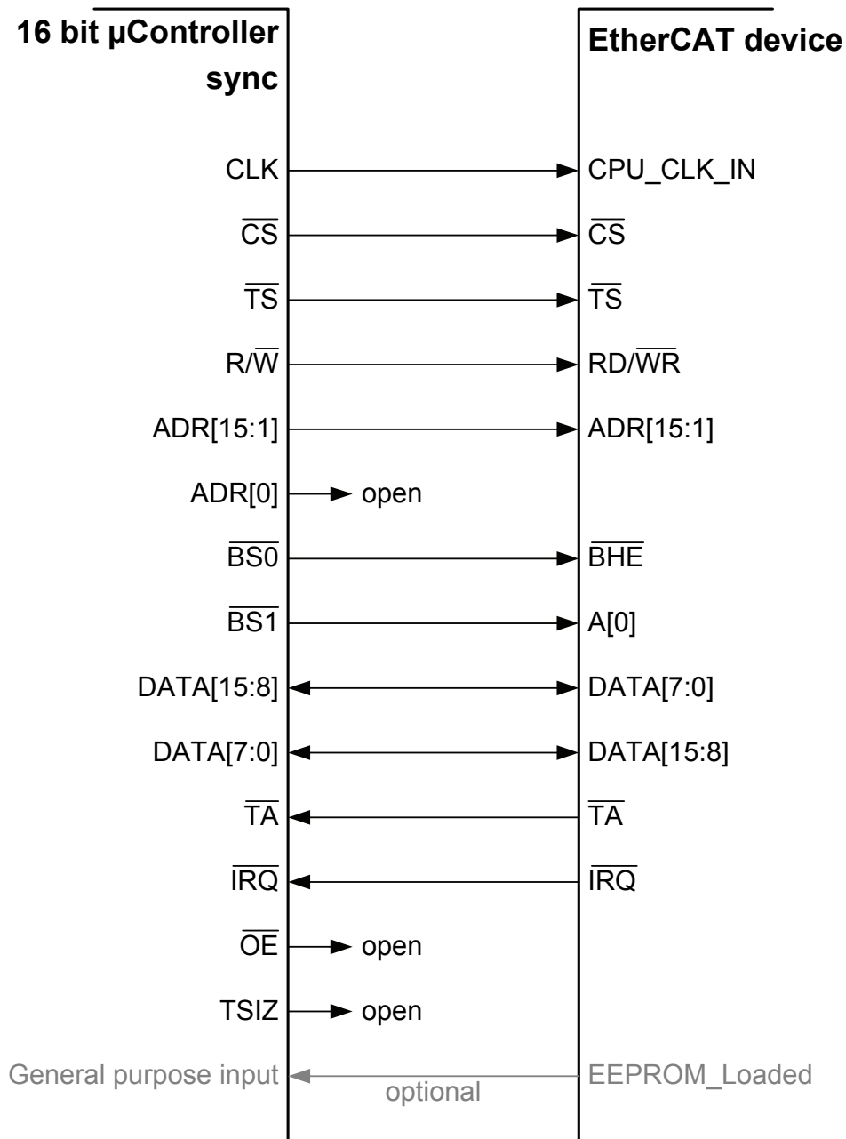
Figure 29: Synchronous 16 bit \mu Controller connection using Byte Select
