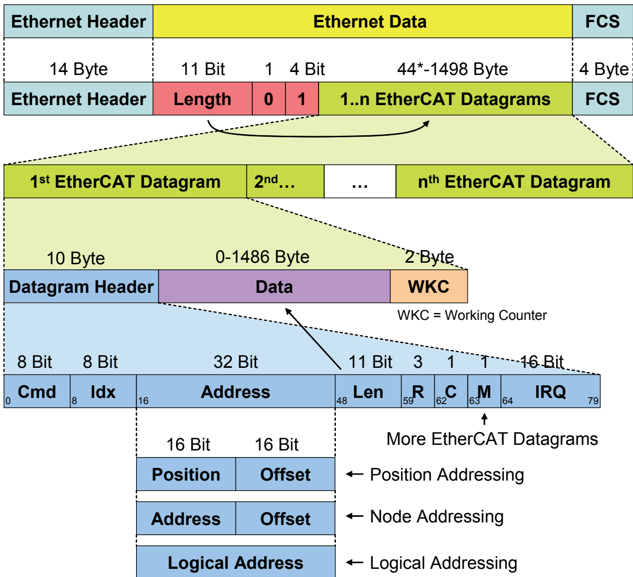
Figure 3: EtherCAT Datagram
