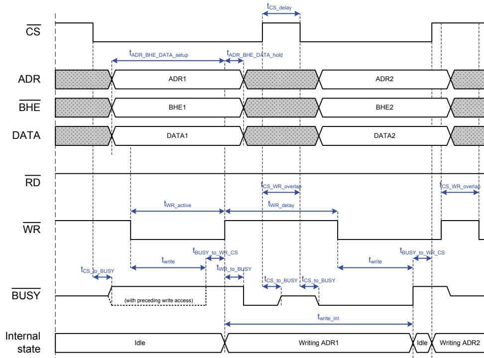
Figure 25: Write access (without preceding write access)
