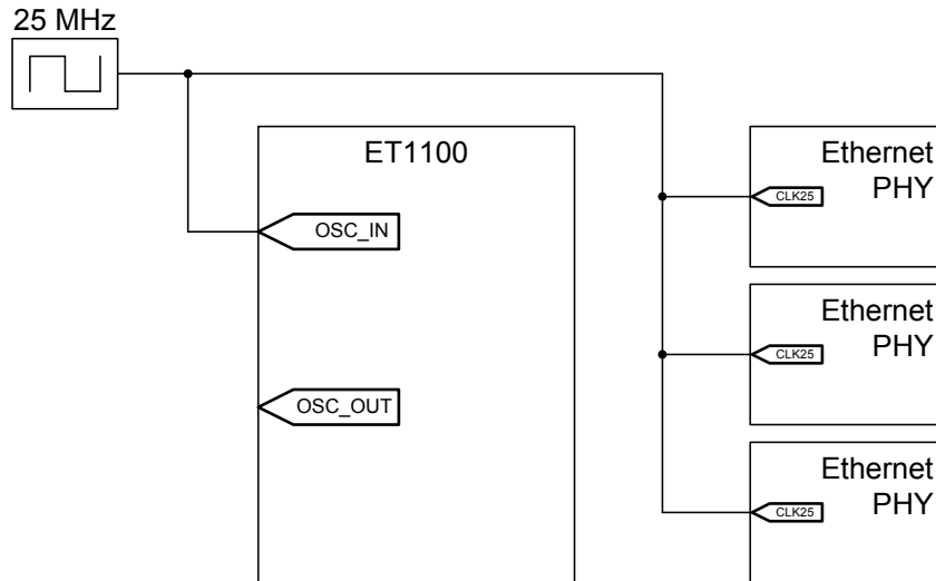
Figure 44: Oscillator clock source for ET1100 and Ethernet PHYs
