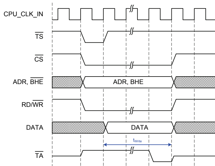
Figure 33: Write access (CS together with TS, Write DATA after CS, CS and TA on rising edge)
