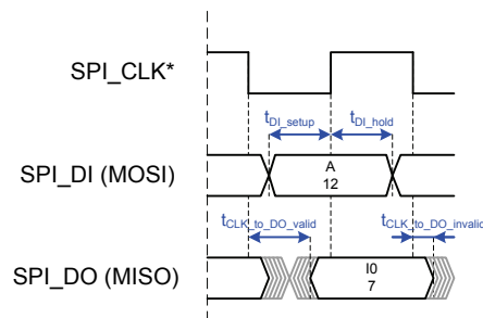
Figure 16: Basic SPI_DI/SPI_DO timing (*refer to timing diagram for relevant edges of SPI_CLK)
