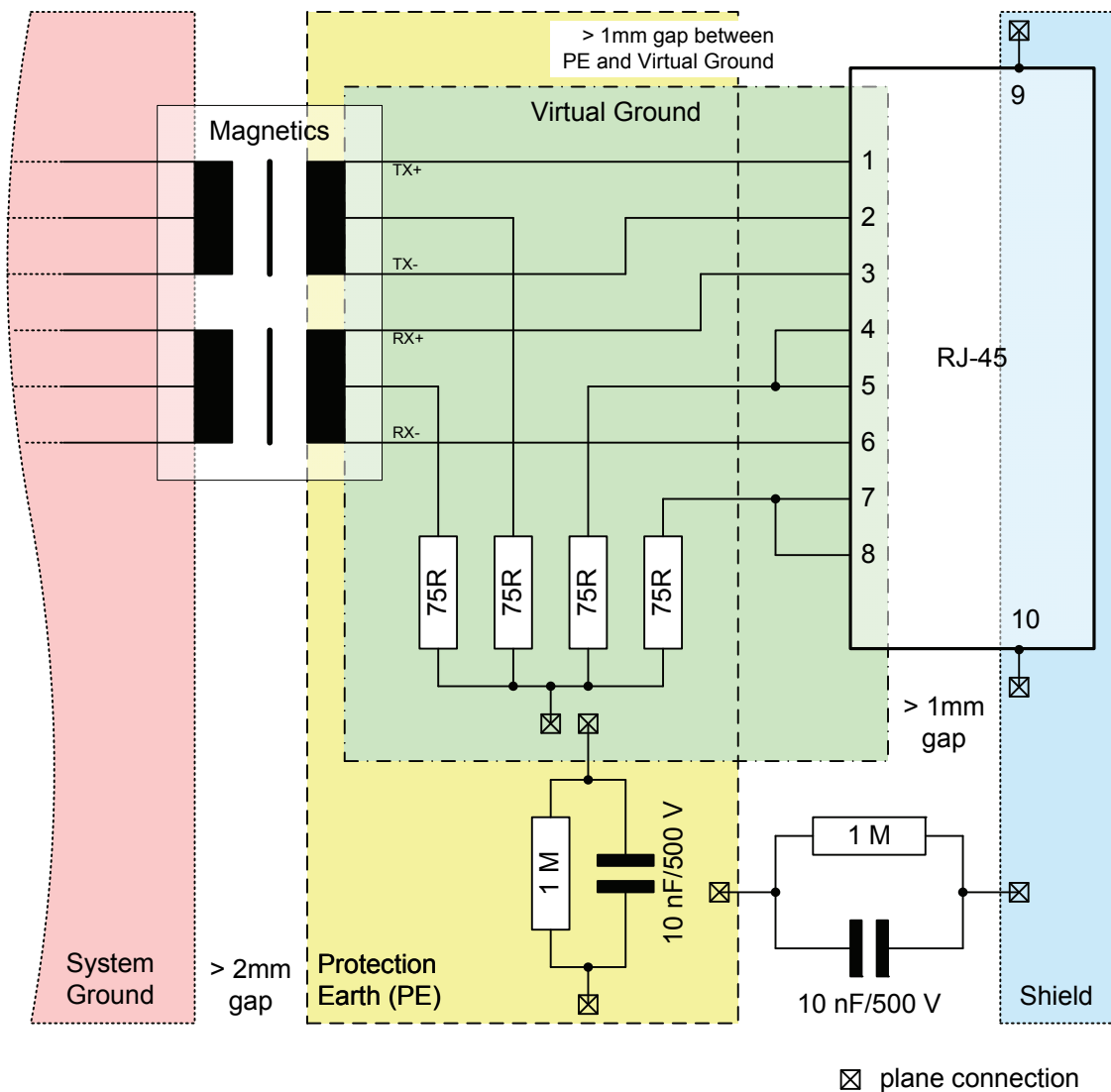
Figure 11: Termination and Grounding Recommendation
