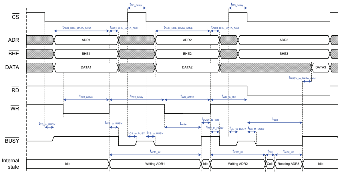
Figure 26: Sequence of two write accesses and a read access
