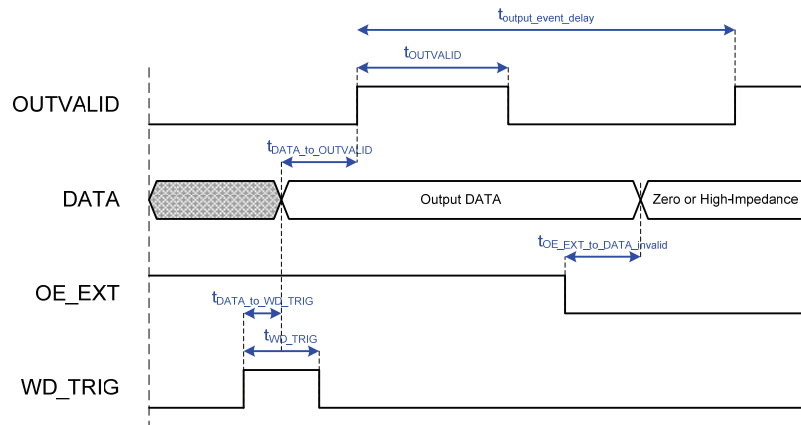
Figure 13: Digital Output timing
