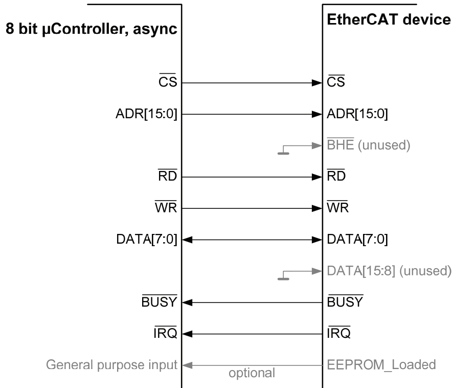
Figure 23: Connection with 8 bit \mu Controllers (BHE and DATA[15:8] should not be left open)
