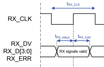
Figure 6: MII timing RX signals
