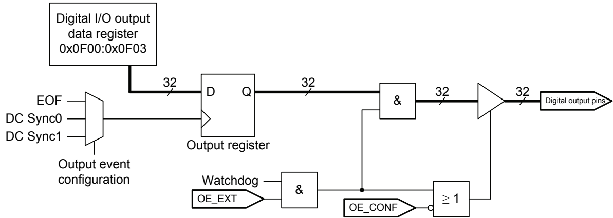
Figure 9: Digital Output Principle Schematic
