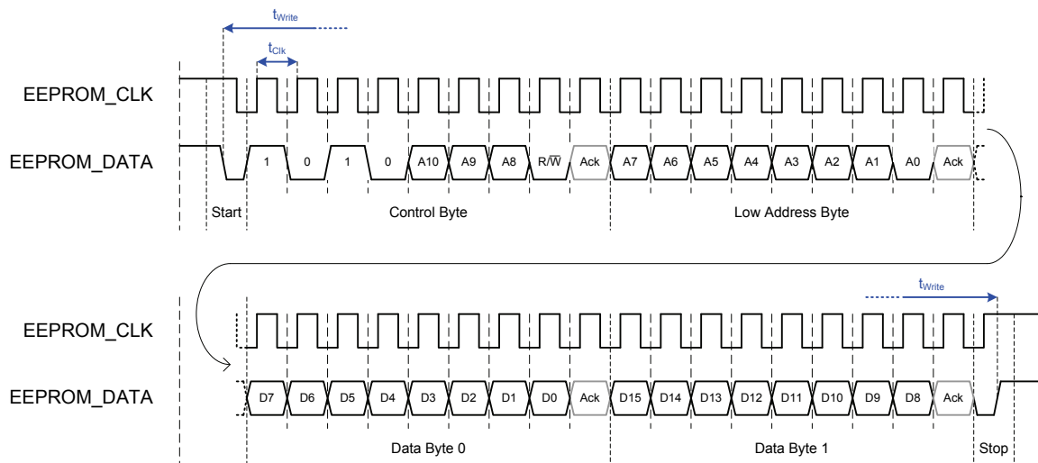
Figure 38: Write access (1 address byte, up to 16 kBit EEPROMs)
