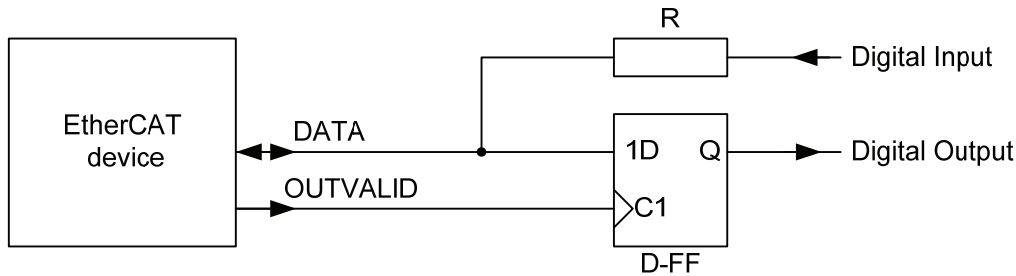
Figure 10: Bidirectional mode: Input/Output connection (R=4.7kΩ recommended)
