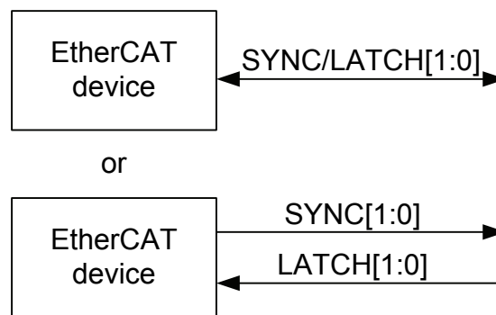
Figure 29: Distributed Clocks signals
