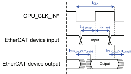
Figure 31: Basic synchronous \mu Controller interface timing (*refer to timing diagram for relevant CPU_CLK_IN edges)
