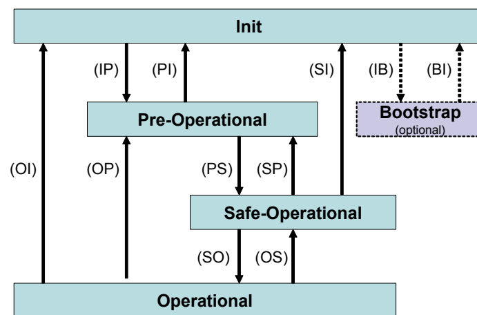
Figure 35: EtherCAT State Machine
