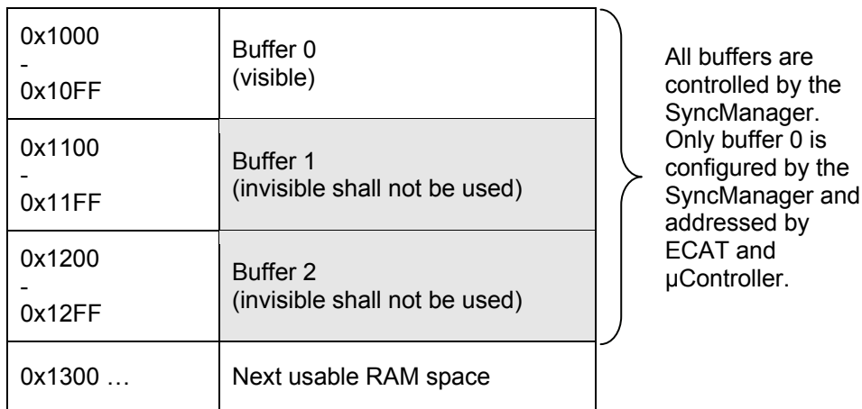
Figure 22: SyncManager Buffer allocation
