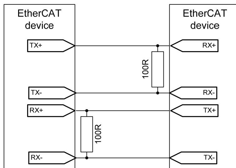
Figure 19: EBUS Connection
