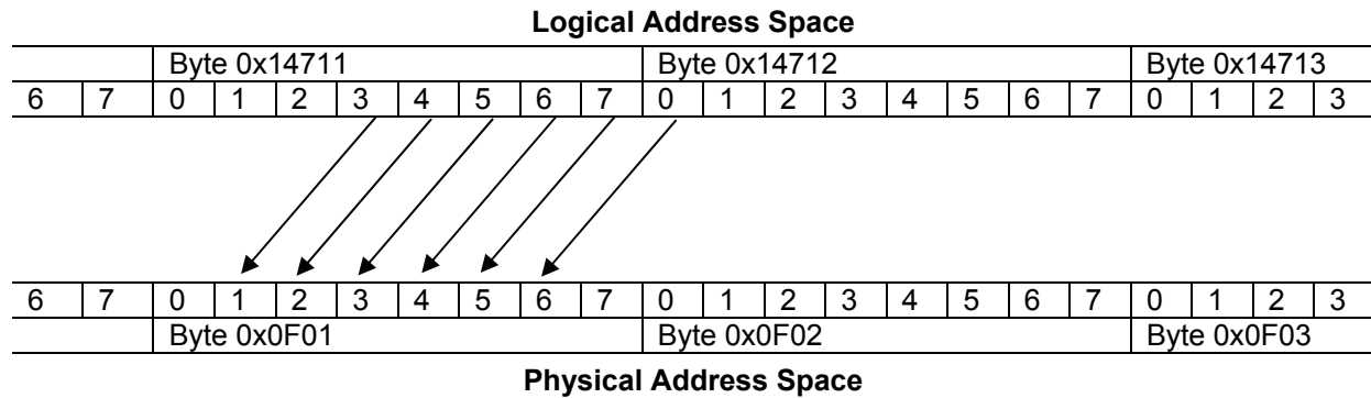
Figure 21: FMMU Mapping Example
