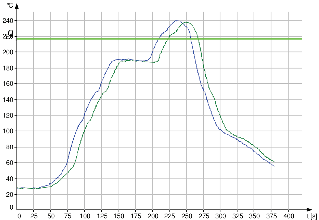
Figure 57: Example Soldering Profiles
