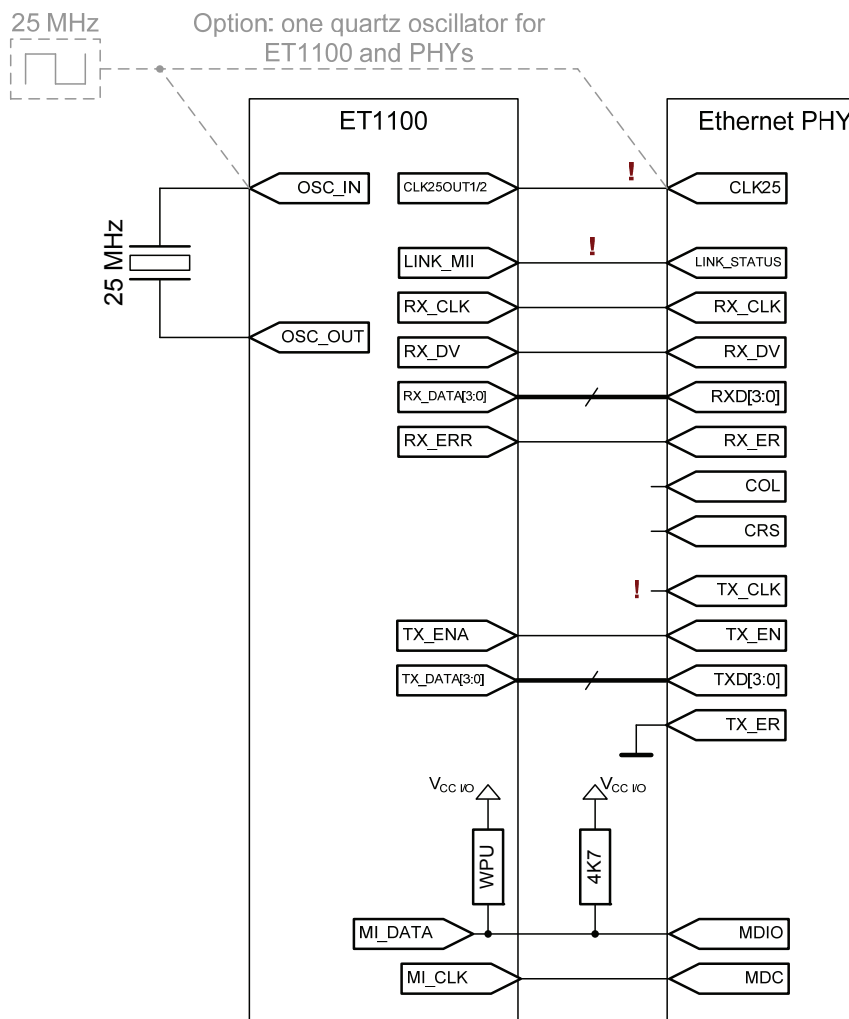
Figure 47: PHY Connection
