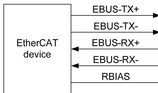
Figure 16: EBUS Interface Signals
