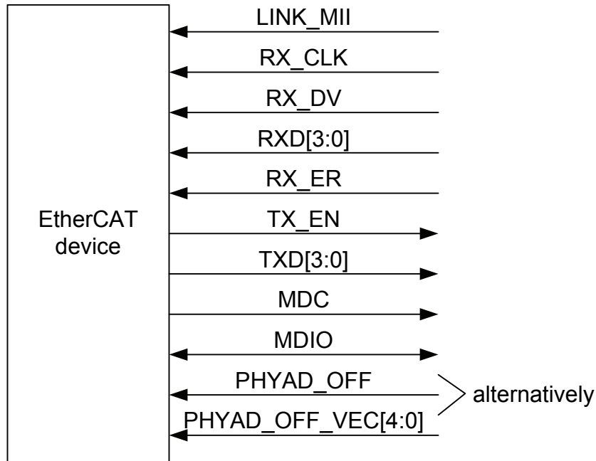
Figure 7: MII Interface signals
