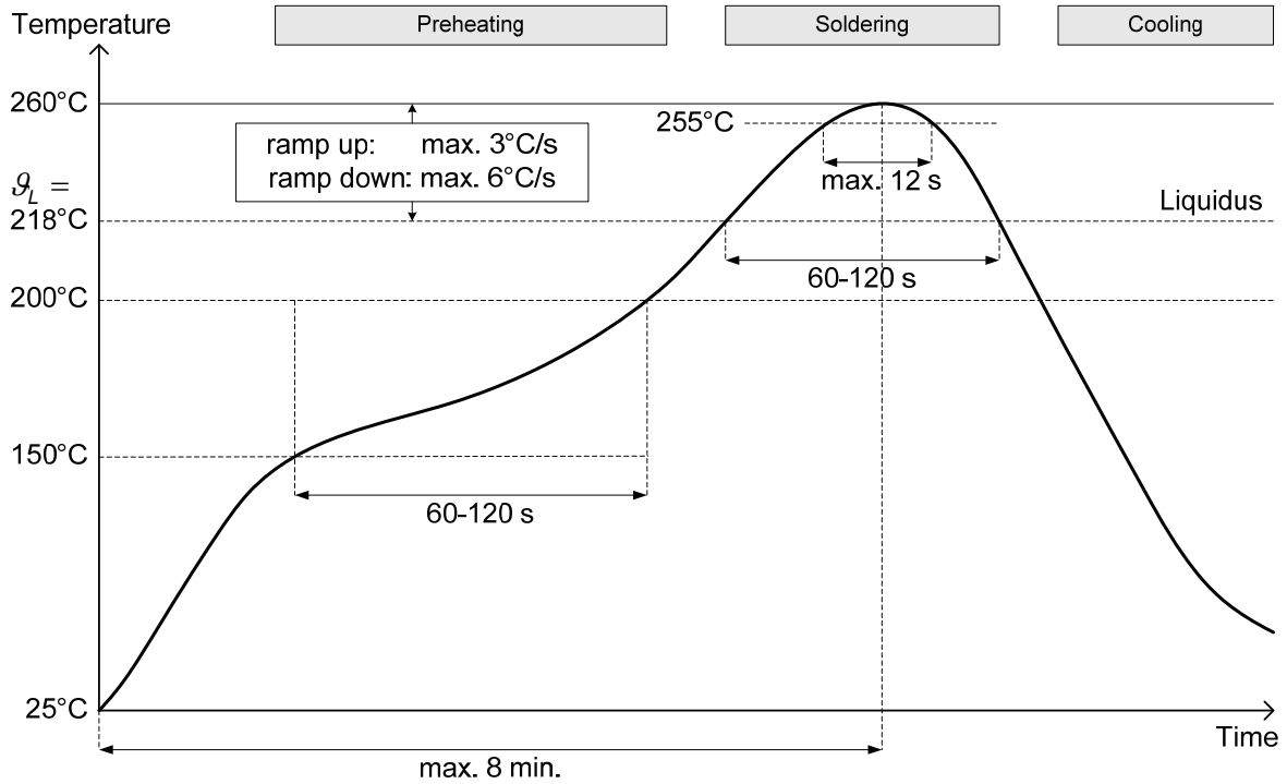
Figure 56: Maximum Soldering Profile
