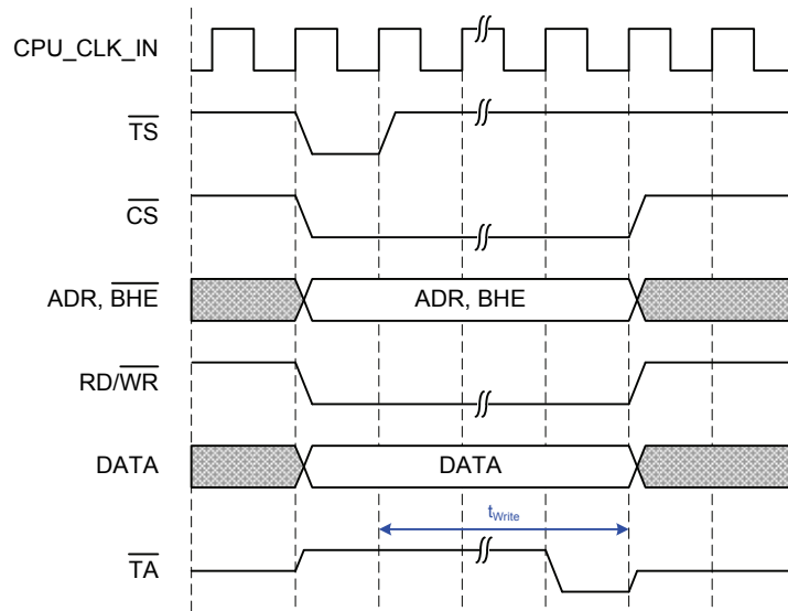
Figure 32: Write access (CS together with TS, Write DATA together with CS, CS and TA on rising edge)
