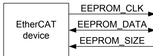
Figure 41: I 2 C EEPROM signals
