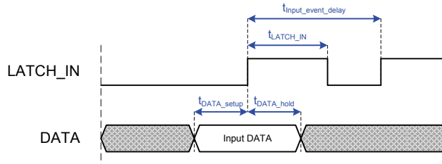
Figure 12: Digital Input: Input data sampled with LATCH_IN
