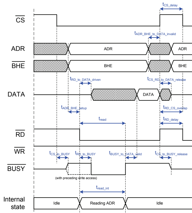
Figure 24: Read access (without preceding write access)
