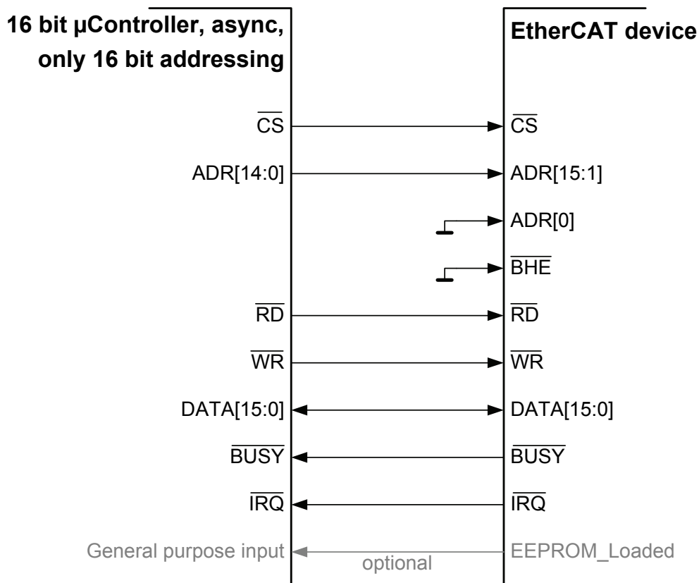
Figure 22: Connection with 16 bit \mu Controllers without byte addressing
