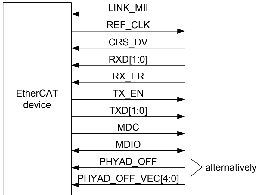
Figure 8: RMI Interface signals
