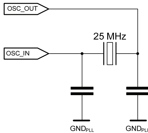
Figure 42: Quartz crystal connection
