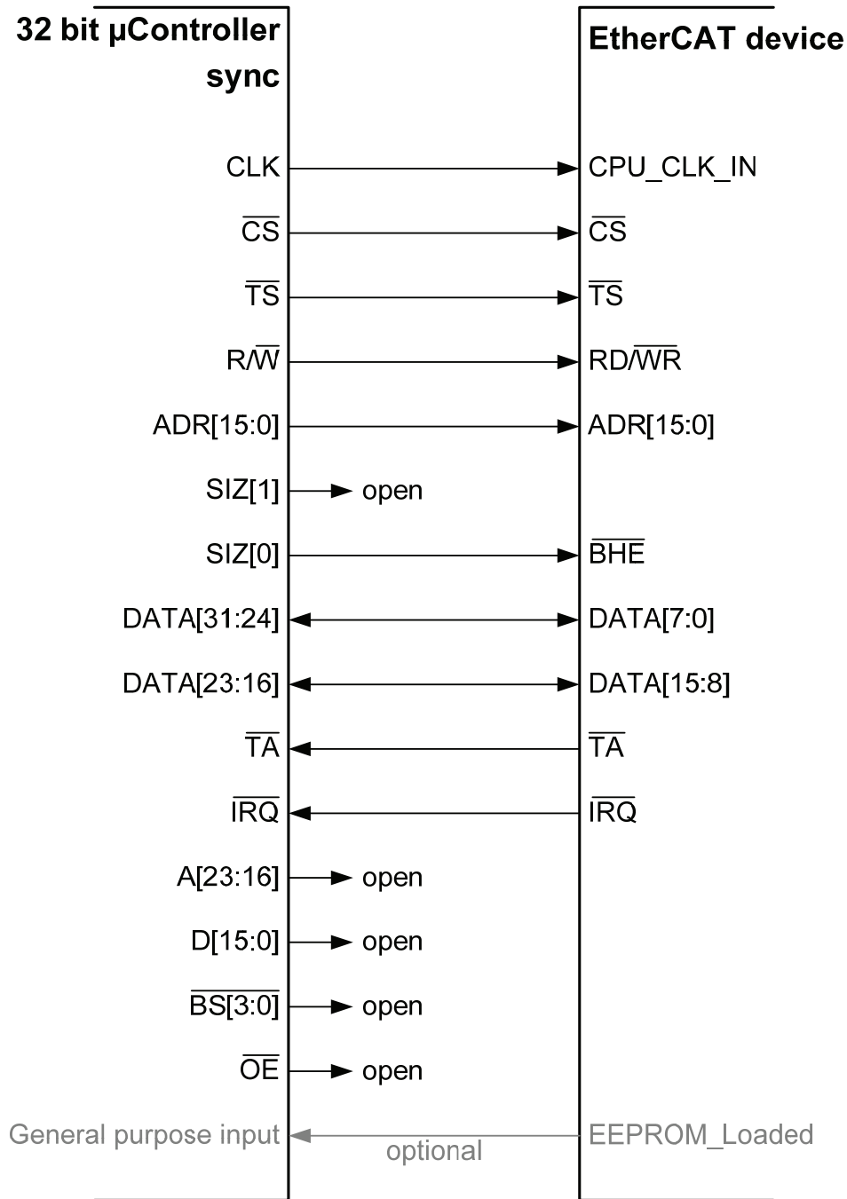
Figure 30: Synchronous 32 bit \mu Controller connection using Transfer Size
