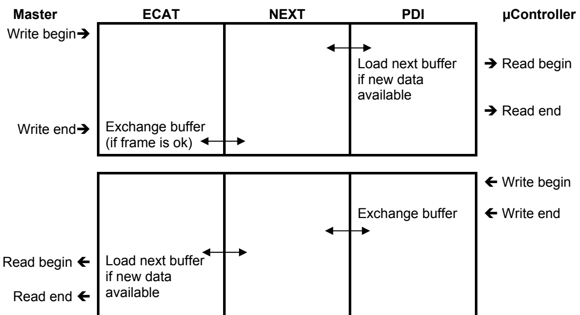
Figure 23: SyncManager Buffered Mode Interaction
