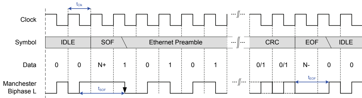
Figure 17: EBUS Protocol
