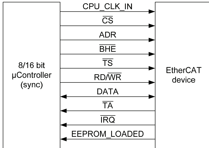
Figure 27: \mu Controller interconnection 4
