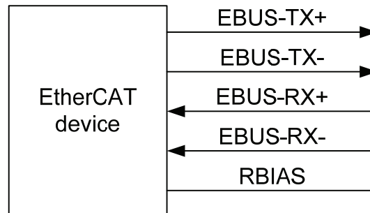
Figure 7: EBUS Interface Signals
