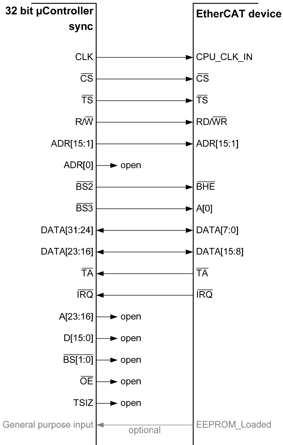
Figure 28: Synchronous 32 bit \mu Controller connection using Byte Select
