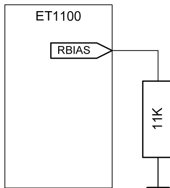
Figure 49: LVDS load resistor
