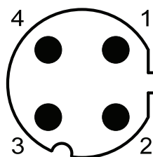
Figure 13: M12 D-code Connector
