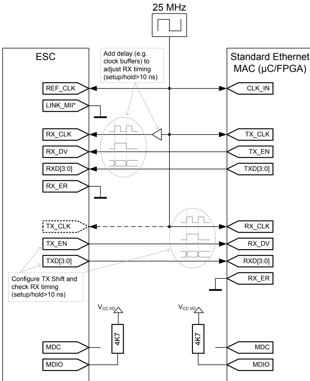
Figure 15: Back-to-Back MII Connection (ESC and standard MAC)
