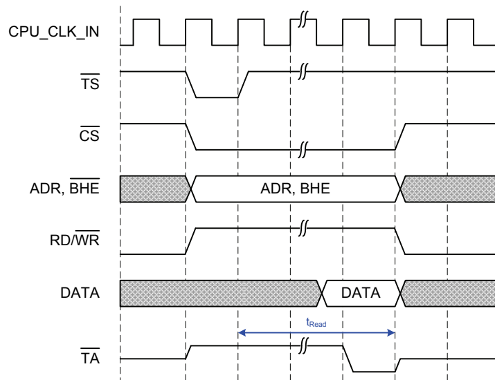
Figure 35: Read access (CS together with TS, CS and TA on rising edge)
