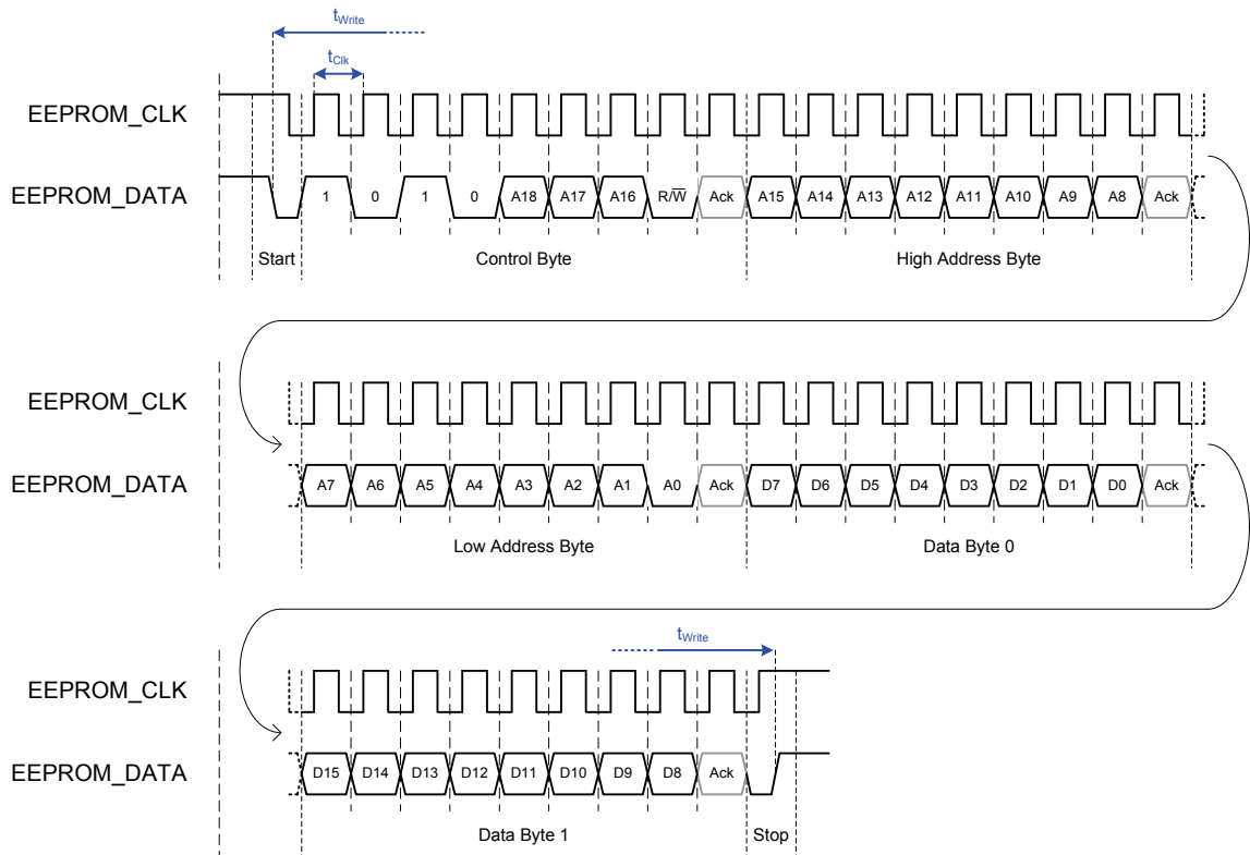
Figure 39: Write access (2 address bytes, 32 kBit - 4 MBit EEPROMs)
