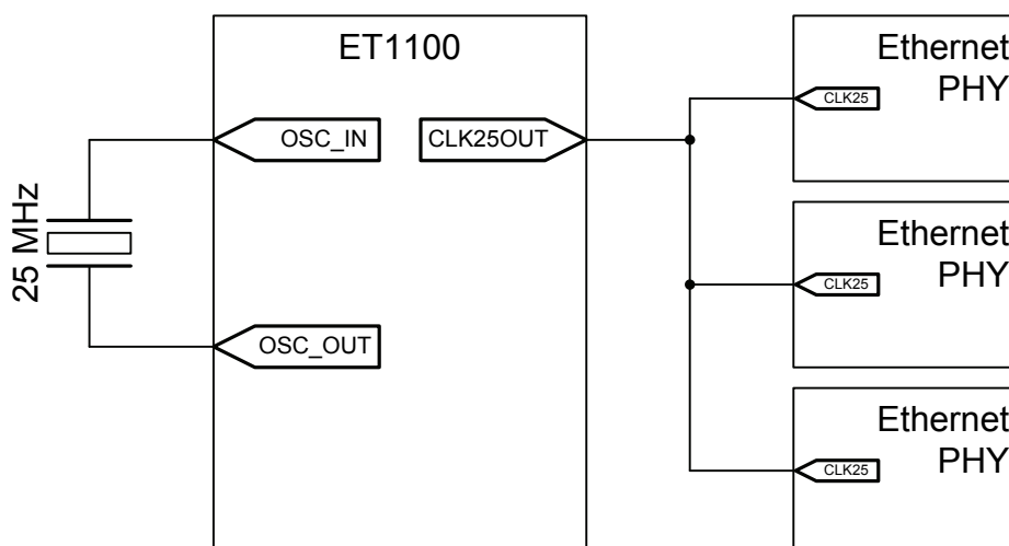
Figure 43: Quartz crystal Clock source for ET1100 and Ethernet PHYs
