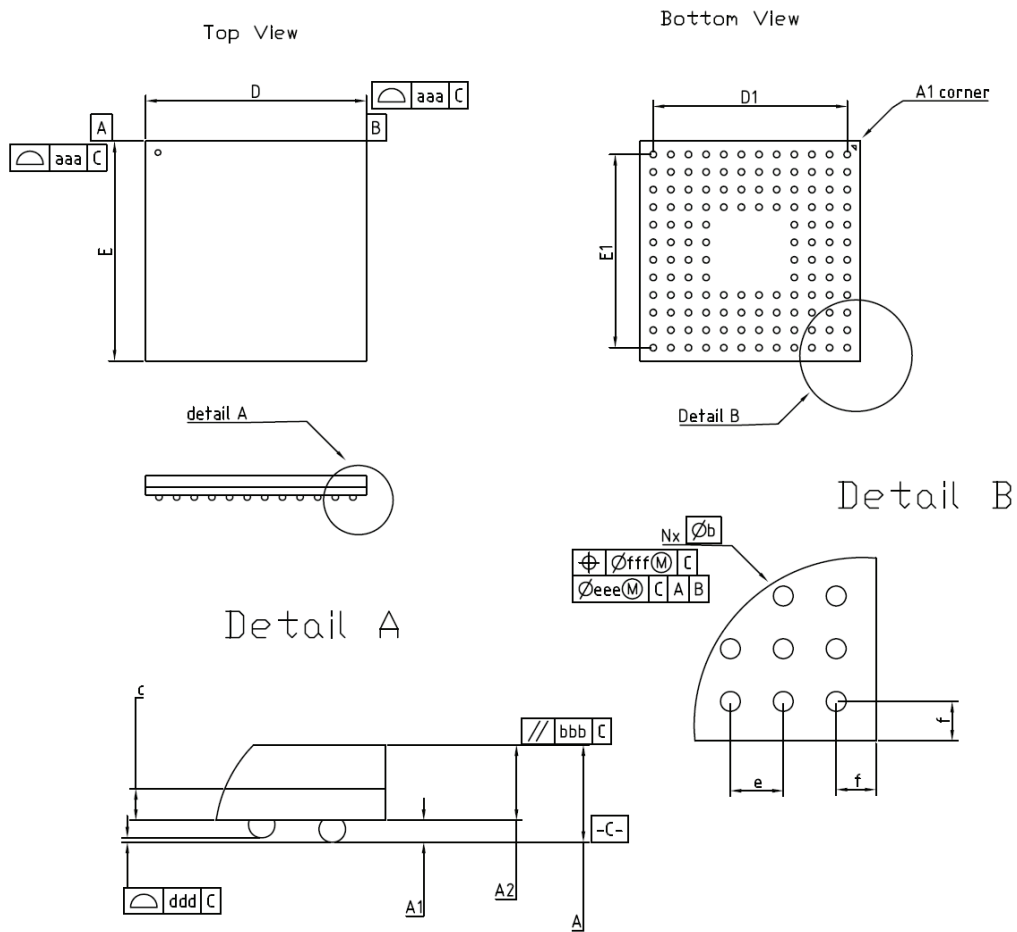
Figure 53: Package Outline
