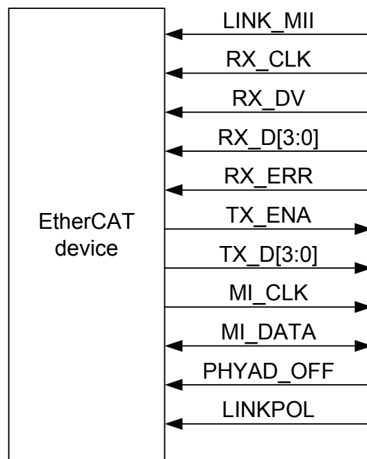
Figure 4: MII Interface signals
