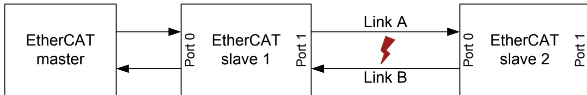
Figure 18: Example EtherCAT Network
